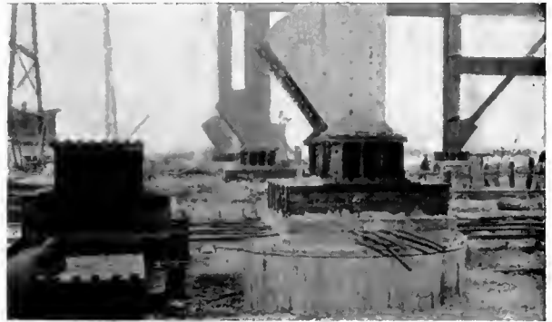
CLOSE-UP OF COLUMN FOOTINGS Showing reinforcing steel at floor beam level
